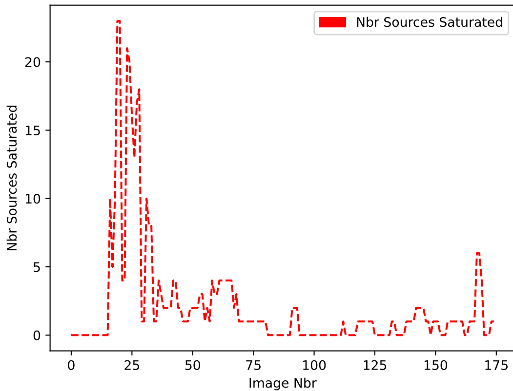
Saturated Sources
