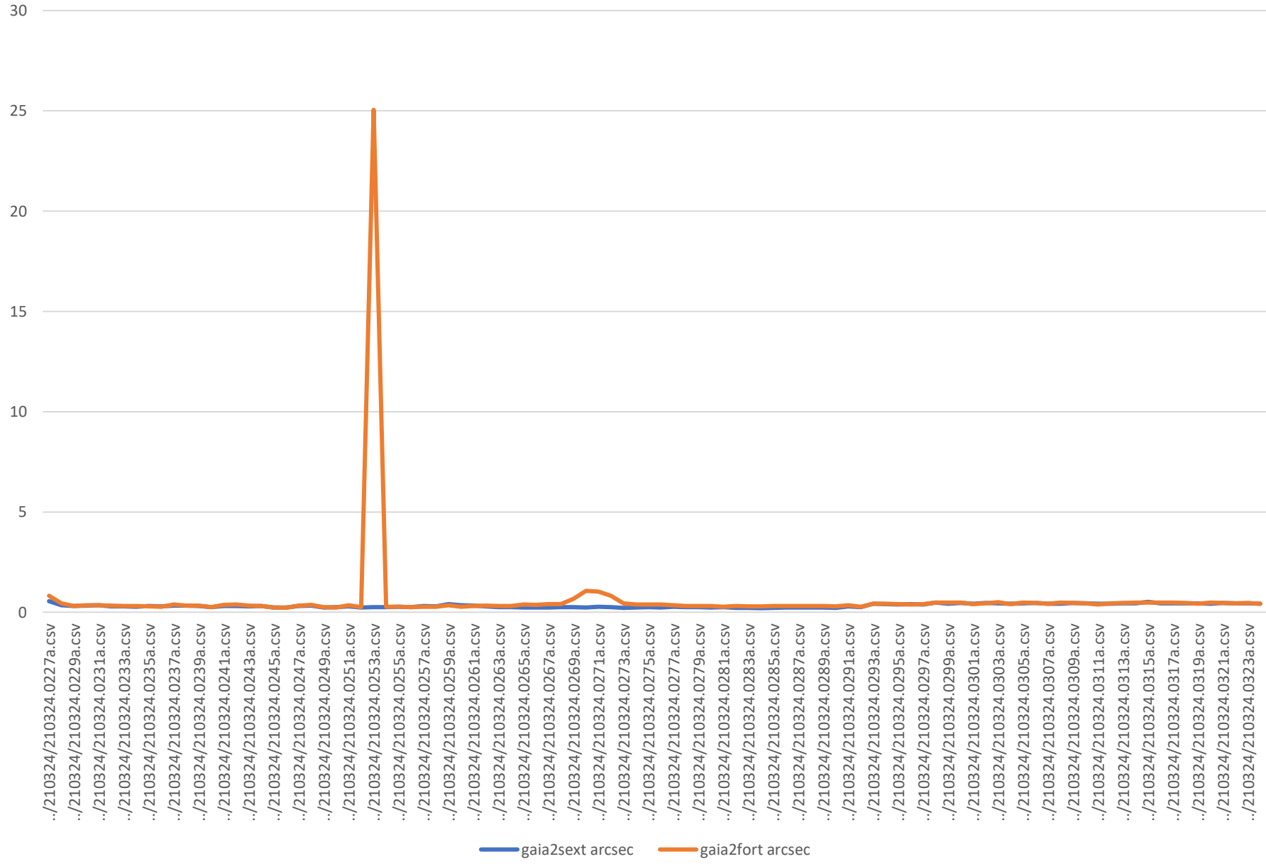
bsm_berry 210324 Gaia to Sext/FORT position
