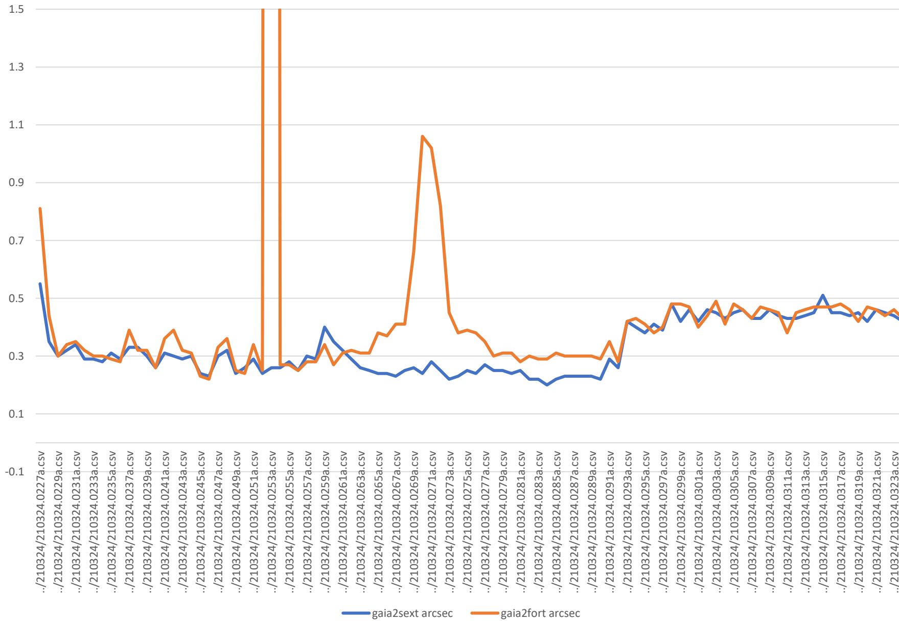
bsm_berry 210324 Gaia to Sext/FORT position
