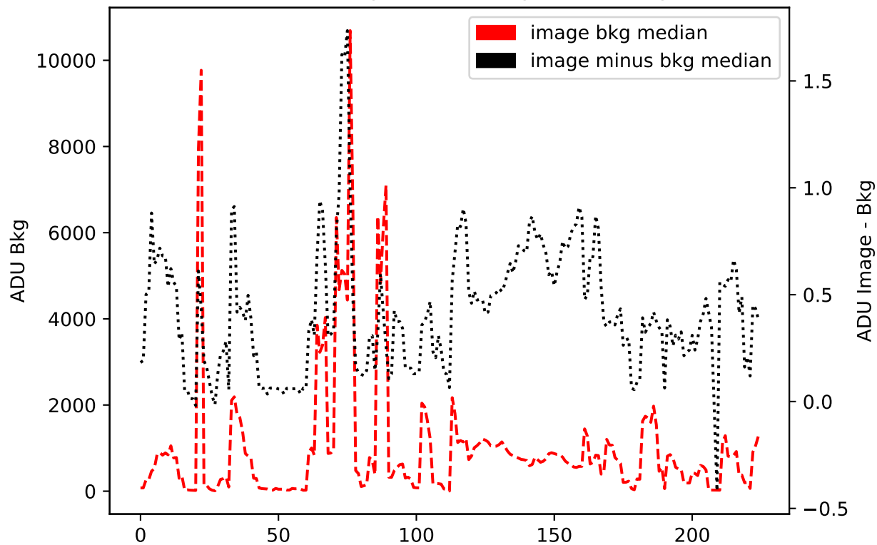
Median ADU of Background and Image Minus Background
