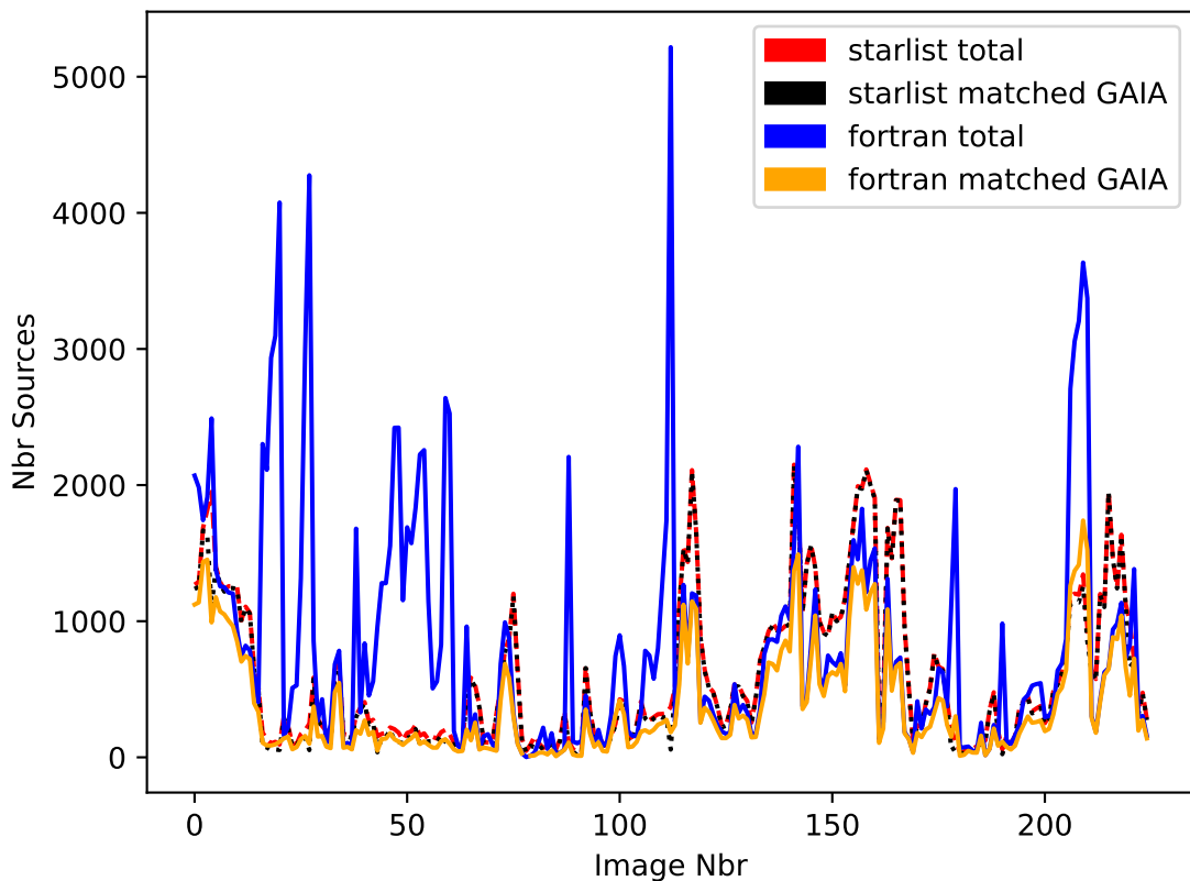
Number of Sources Total and Valid
