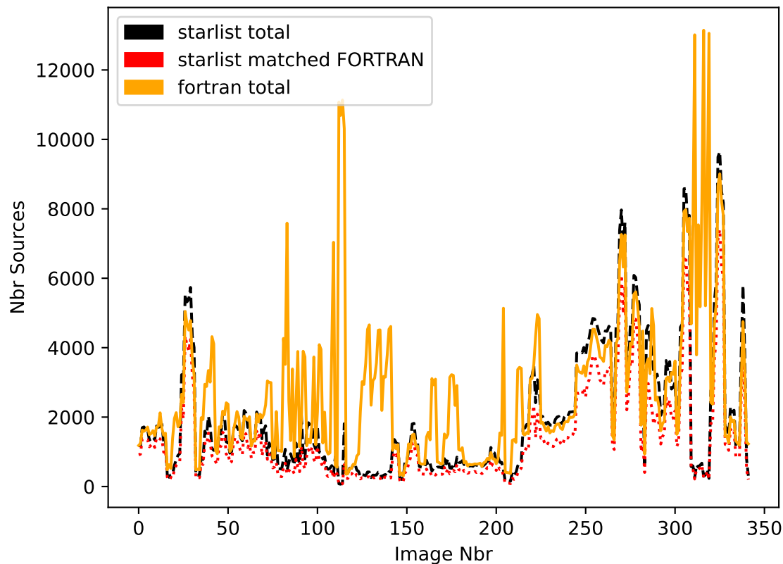
Number of Sources In Both FORTRAN and Starlist
