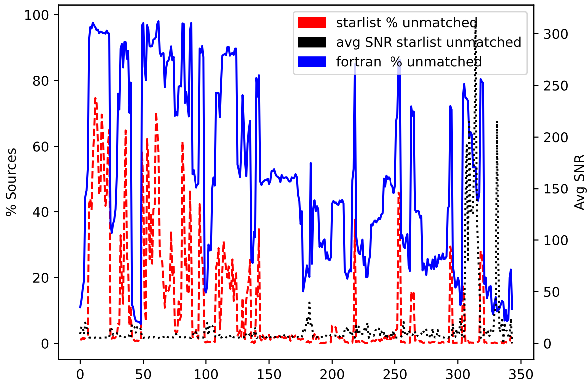
% Sources Unmatched to GAIA
