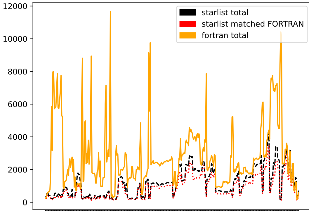
Number of Sources In Both FORTRAN and Starlist
