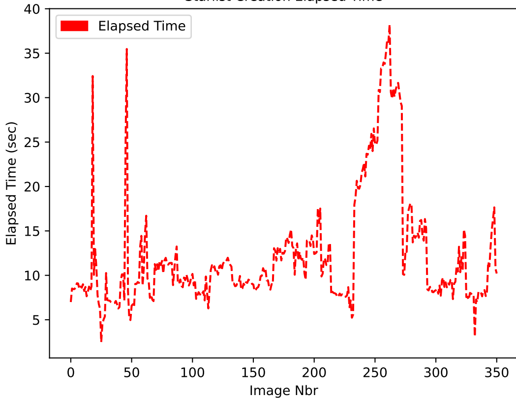
Starlist Creation Elapsed Time
