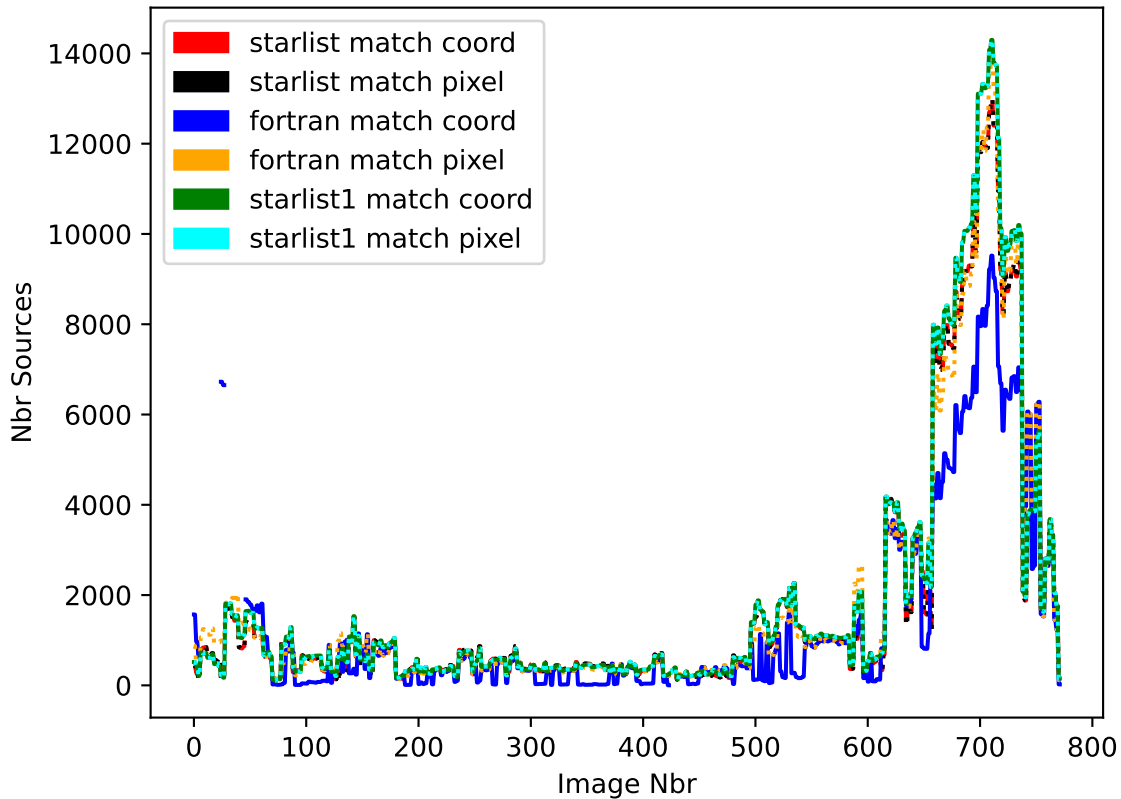
RA/DEC vs Pixel Matching GAIA - X/Y and RA/DEC Ok?
