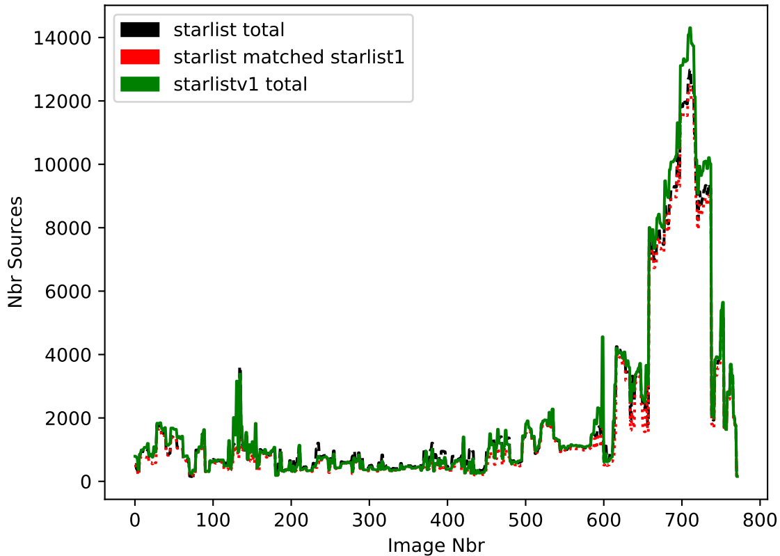
Number of Sources In Both Starlist1 and Starlist
