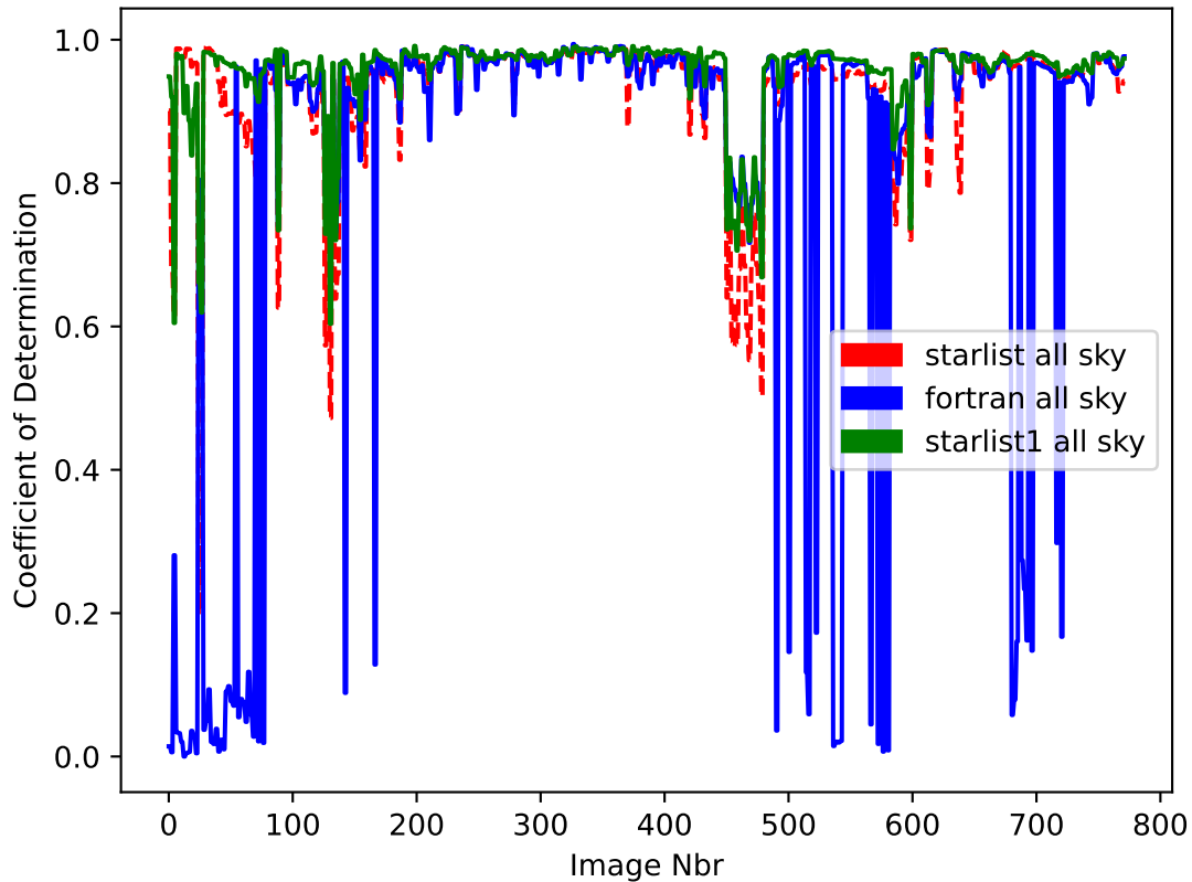
Instr Mag Estimate of Std Mag Fit
