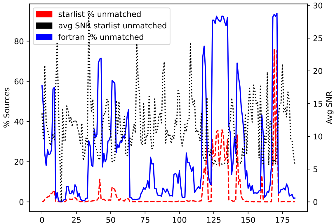
% Sources Unmatched to GAIA
